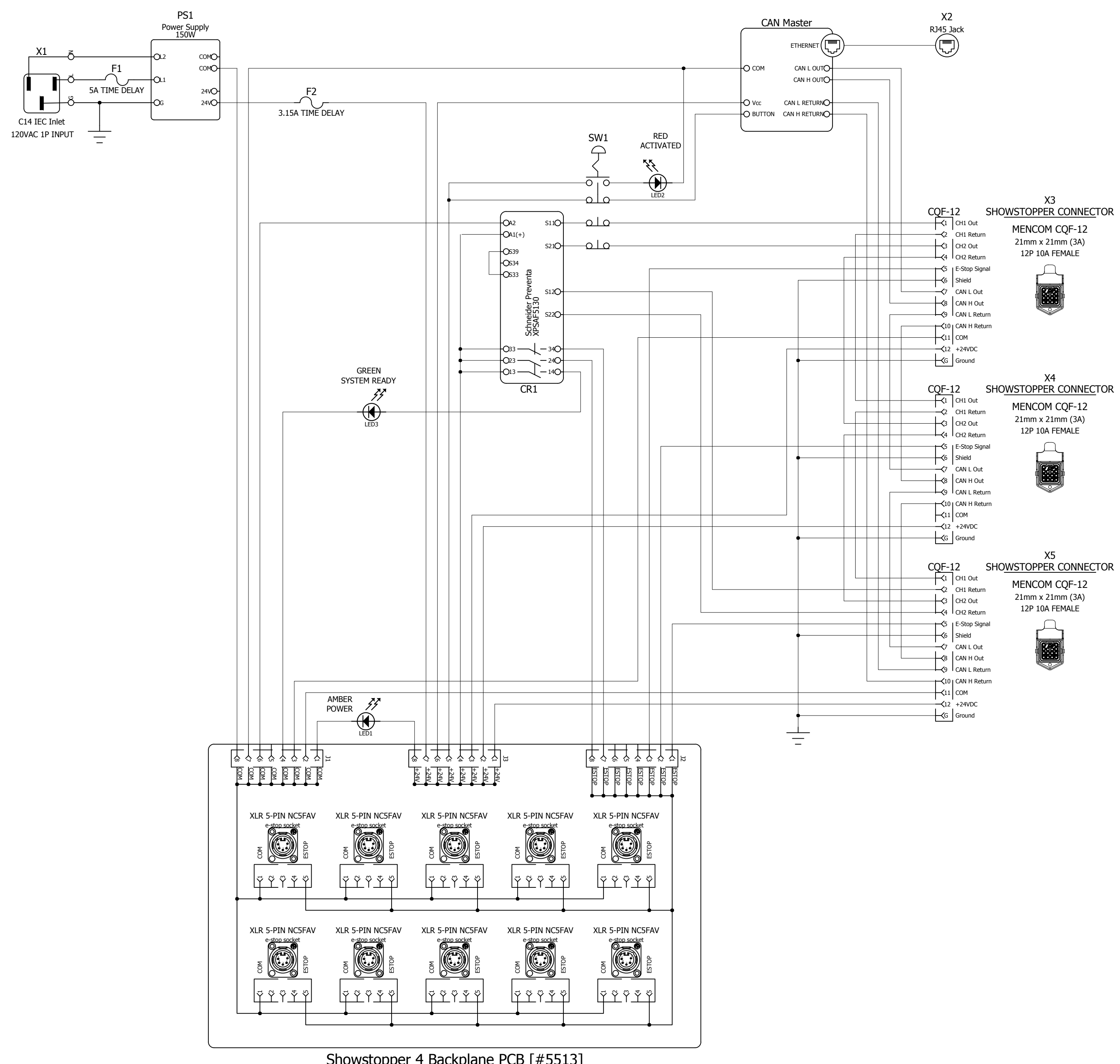
Showstopper 4 Backplane PCB [#5513]
