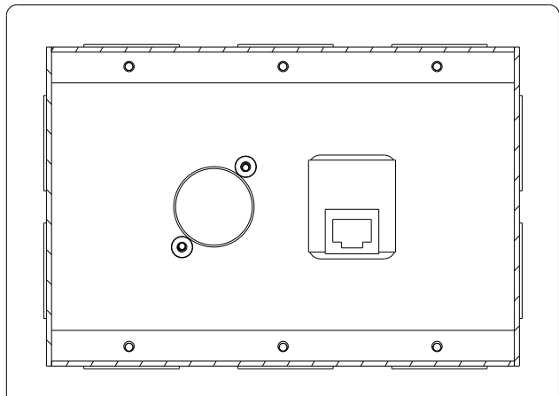
INTERIOR VIEW
