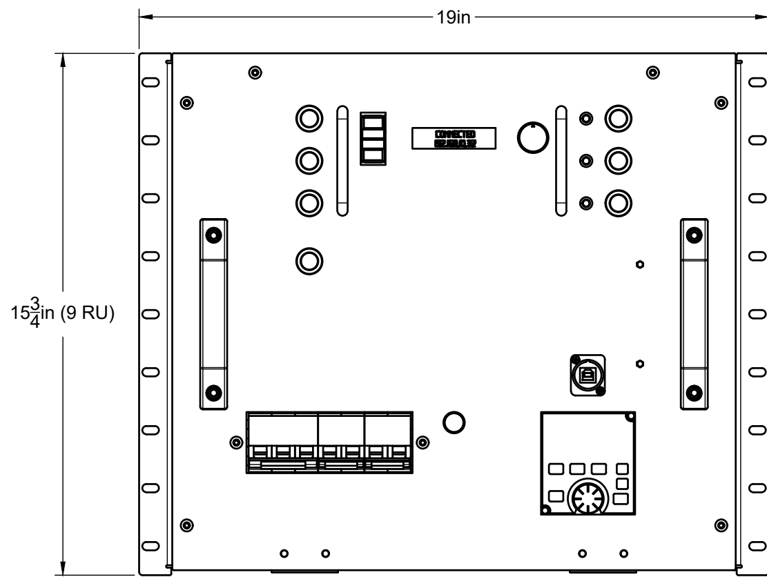
Front View
